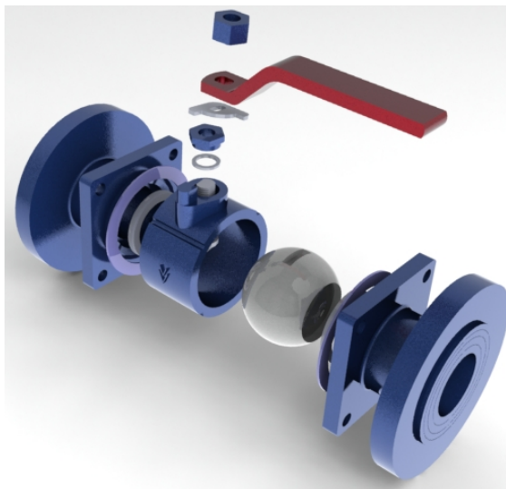
Exploded View
